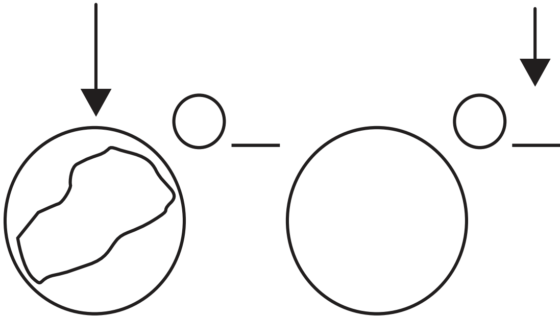
Asteroid
