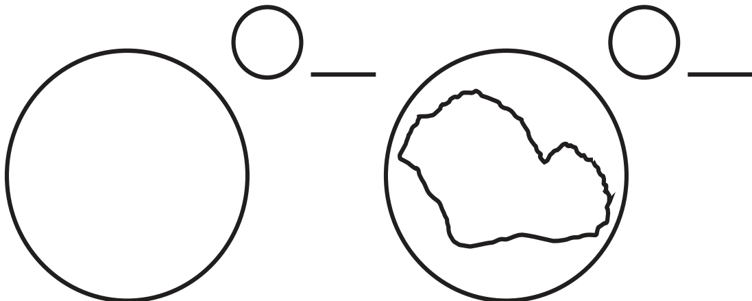
Neptune
